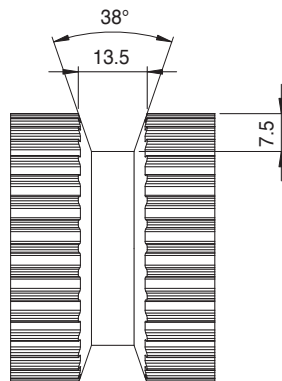
Pulleys profile K13
